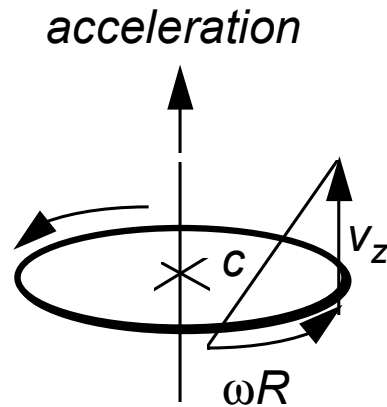
Figure 3. Geometry for calculating the increase of inertial mass with velocity when an electron (or proton) acquires kinetic energy as a result of acceleration. The rim velocity of charge in the ring's own electric fields is maintained at c , the speed of light.
