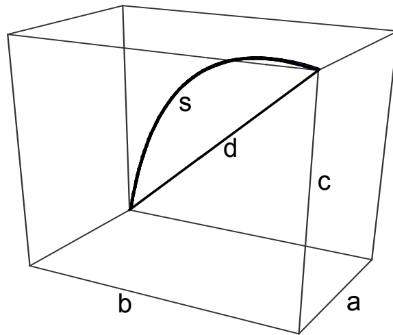
Figure 1. Illustration of a path in “curved space” that is longer than a straight line in Euclidean space. Einstein disregarded the Theorem of Pythagoras. His STR attempts to make s^2 equivalent to d^2 = a^2 + b^2 + c^2 .
