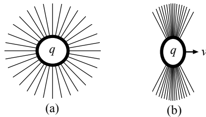
Figure 2. Electric Field Intensity of Charged Sphere, from equation (IV). Part (a) shows the field lines for the charge at rest. Part (b) shows the field lines for the same charge moving at a velocity 0.94c , so that \beta = 0.94 .
